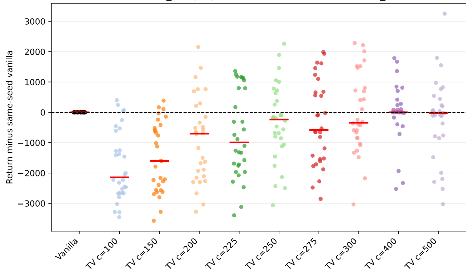
Walker2d-v5 mass_damping factor=0.5: seed scatter (vanilla_subtracted)
