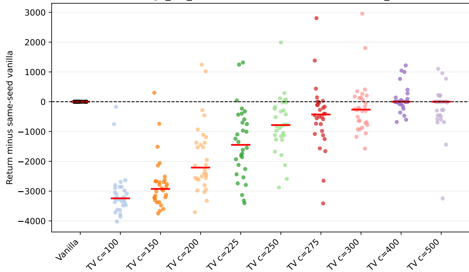
Walker2d-v5 thigh_left_mass factor=0.5: seed scatter (vanilla_subtracted)
