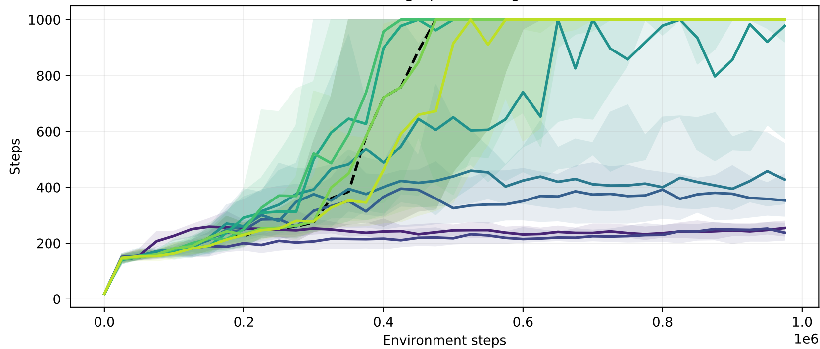
Training episode length
