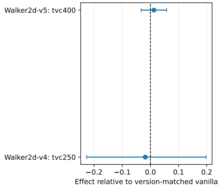
Axis-balanced CVaR20
