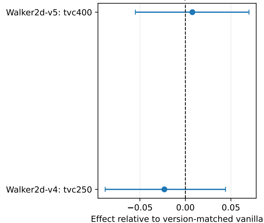
Reliability AUC
