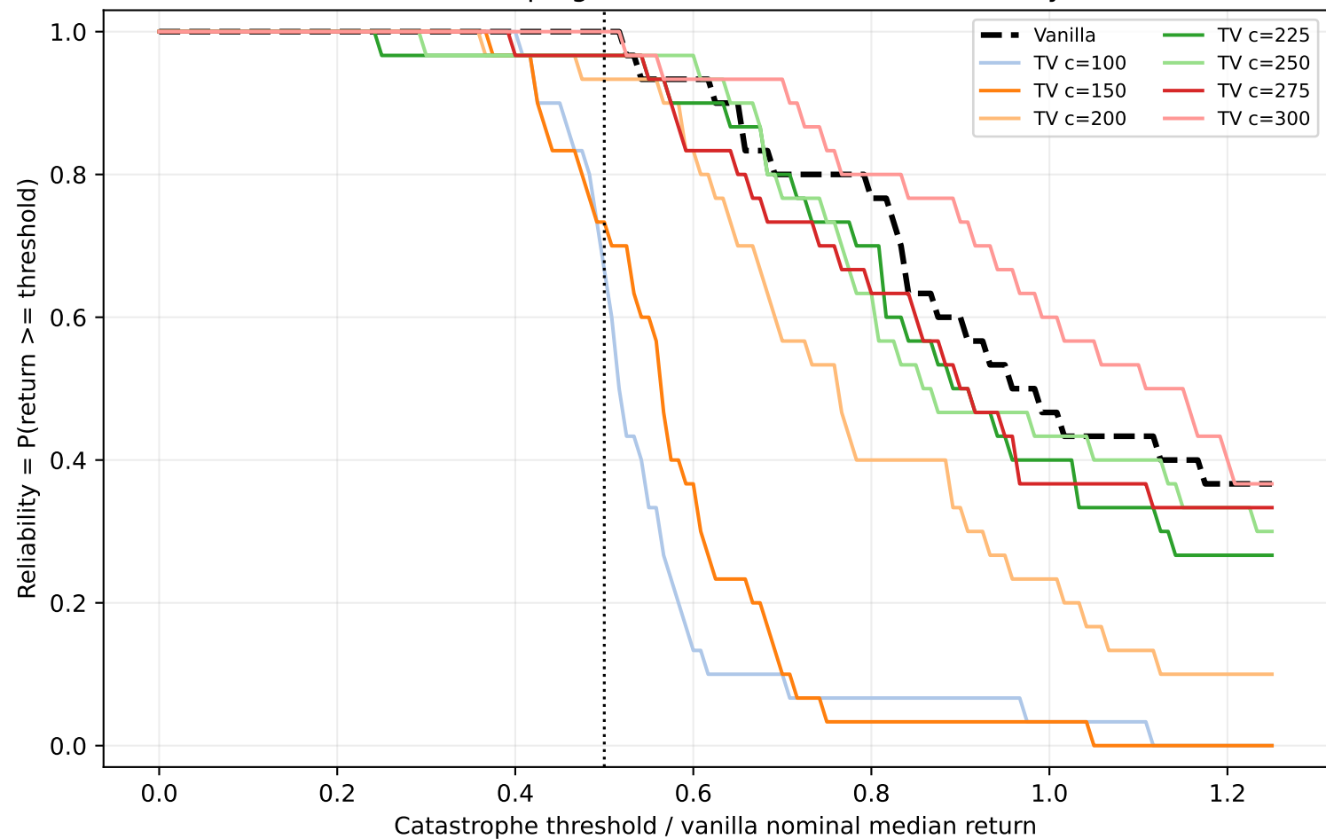
Walker2d-v4 damping factor=0.5: robustness reliability curve
