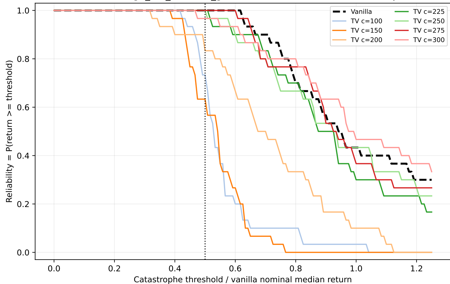
Walker2d-v4 thigh_left_actuator_gain factor=0.5: robustness reliability curve
