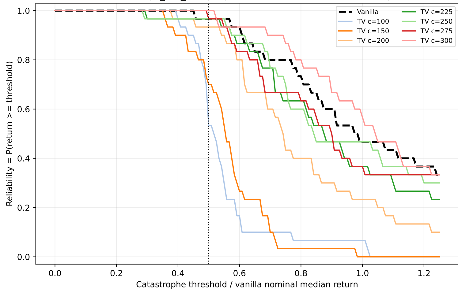
Walker2d-v4 thigh_left_damping factor=0.5: robustness reliability curve
