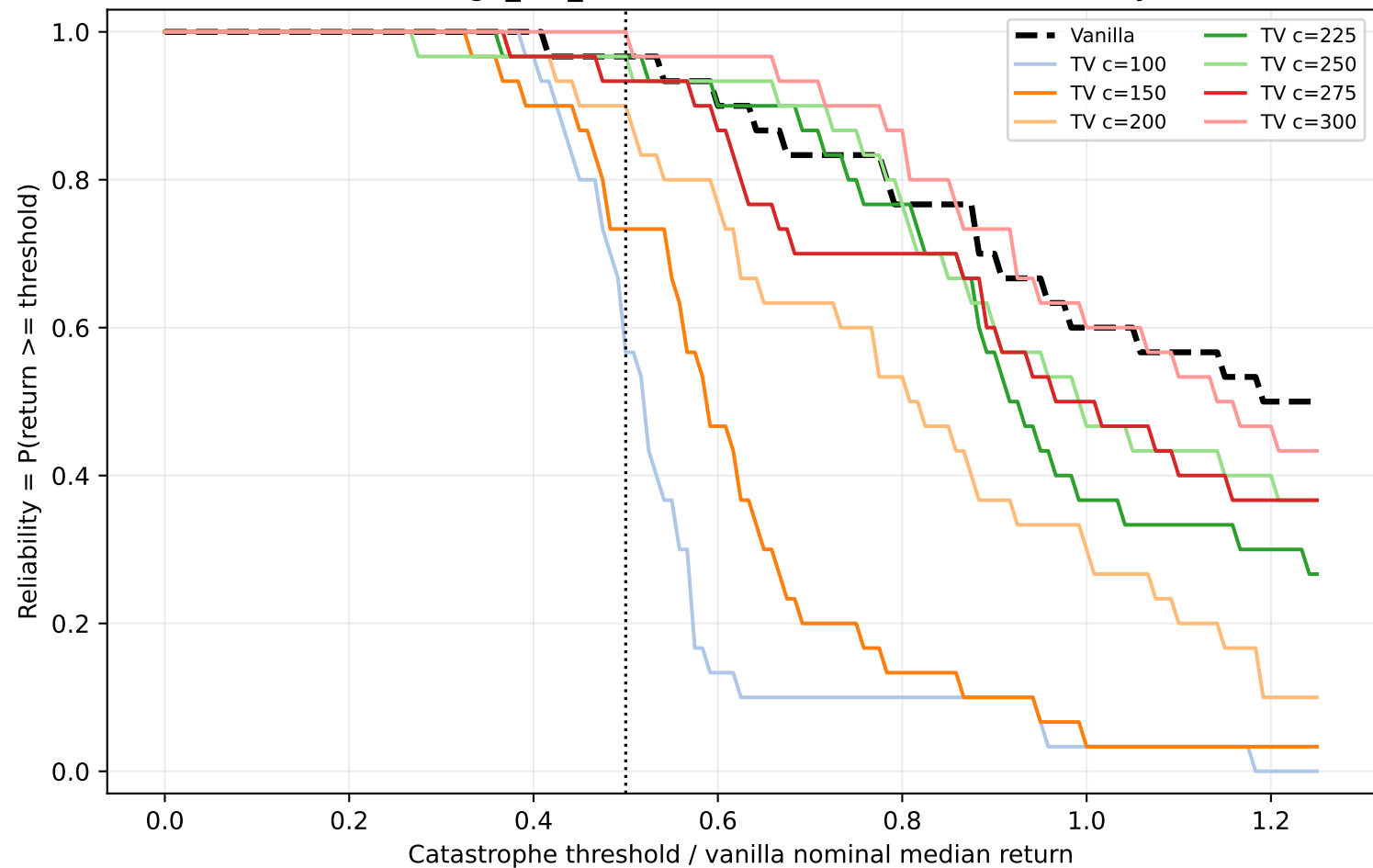
Walker2d-v4 thigh_left_mass factor=0.5: robustness reliability curve
