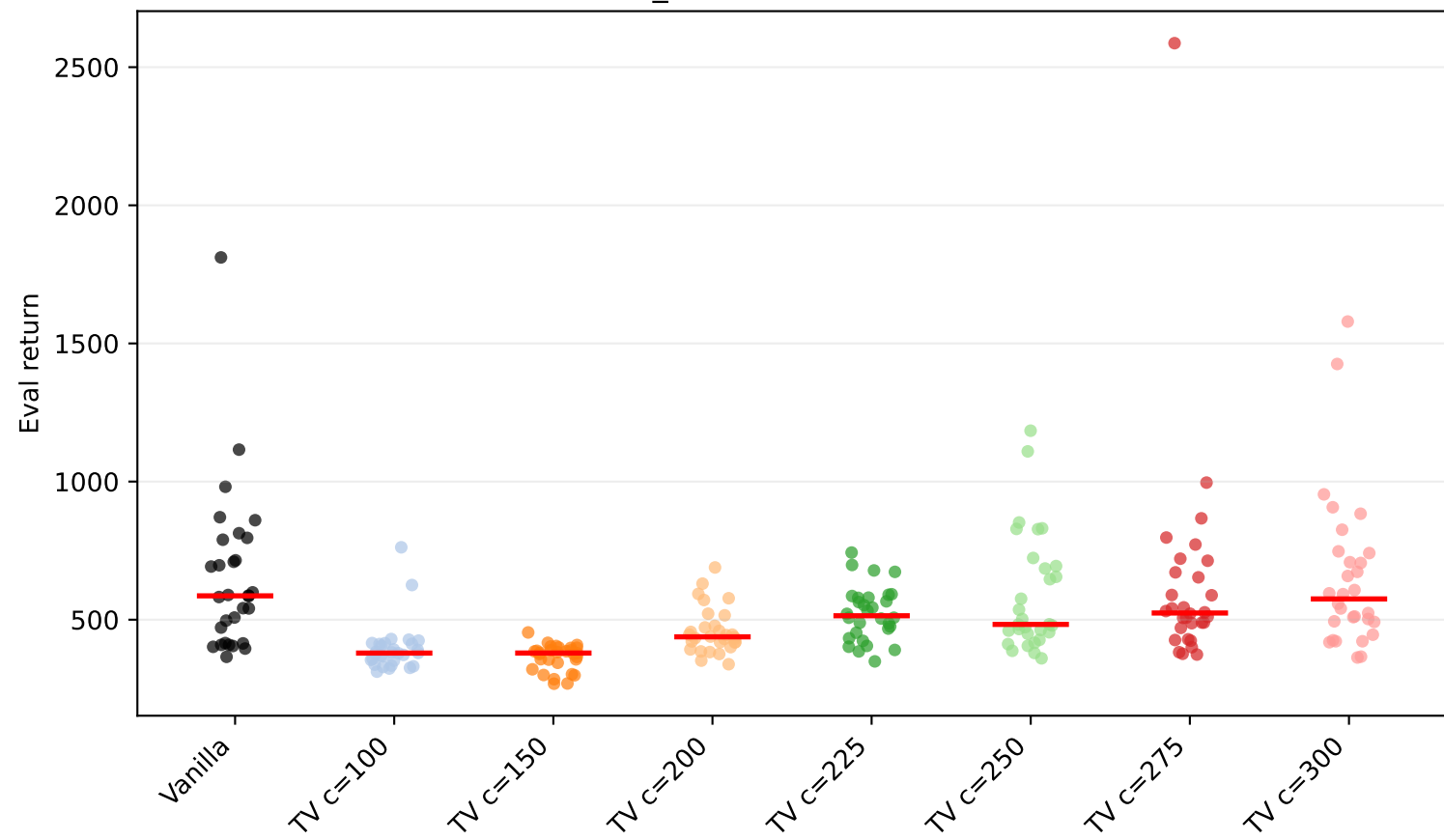
Walker2d-v4 action_noise=0.5: seed scatter (raw)
