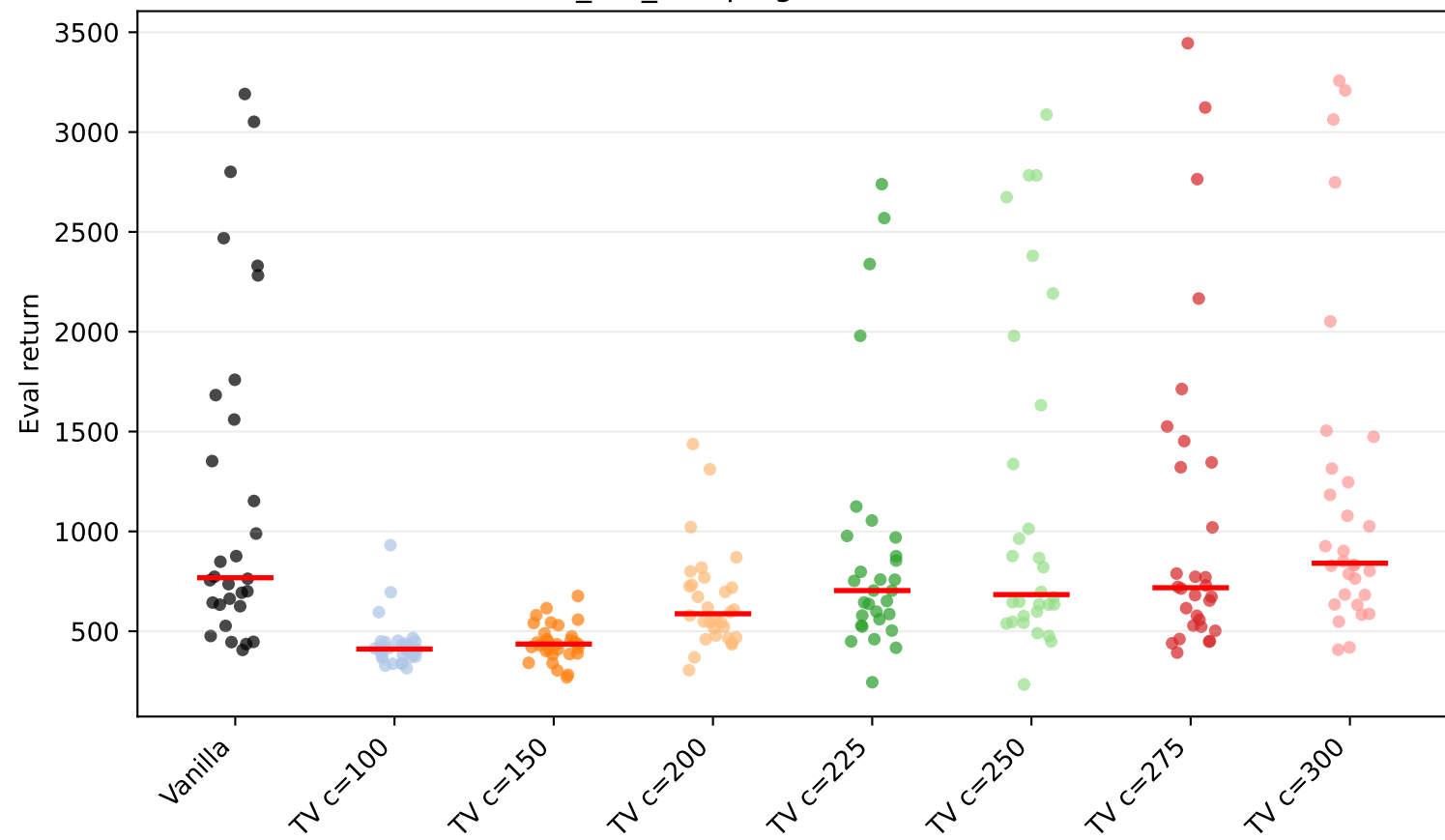
Walker2d-v4 foot_left_damping factor=0.5: seed scatter (raw)
