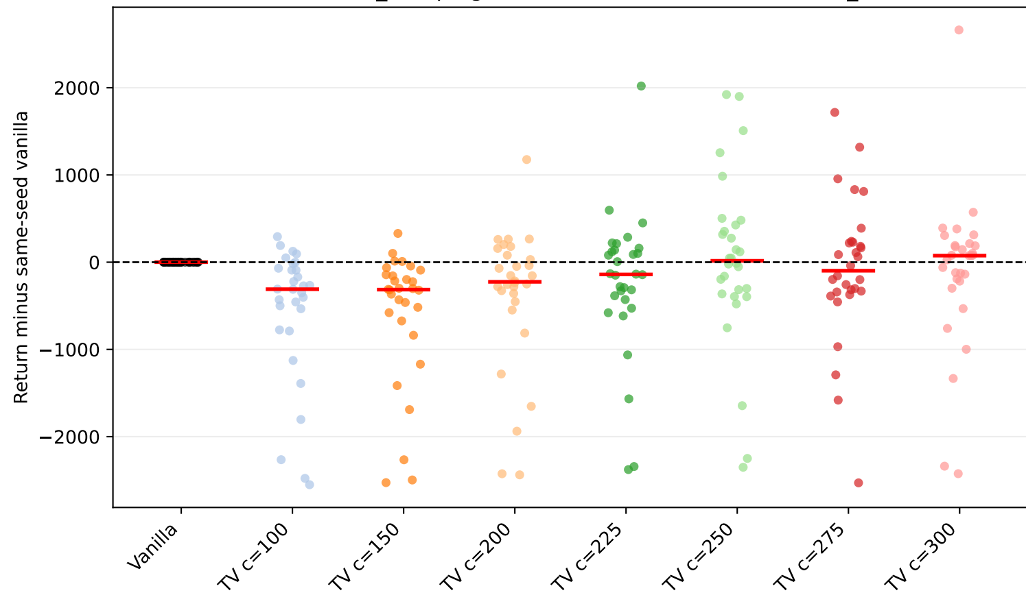
Walker2d-v4 friction_damping factor=0.5: seed scatter (vanilla_subtracted)
