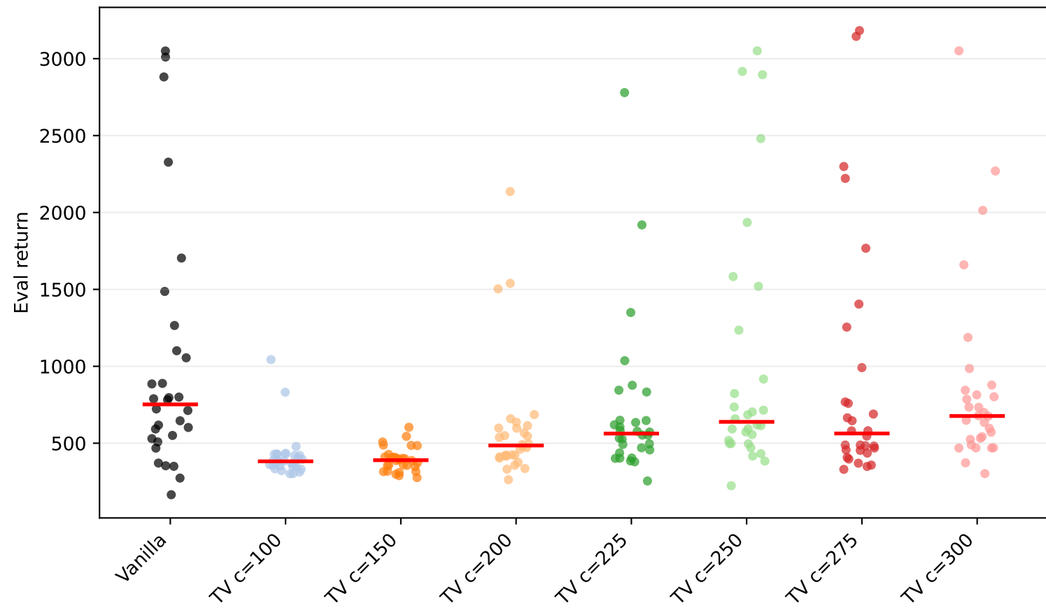
Walker2d-v4 friction factor=0.5: seed scatter (raw)
