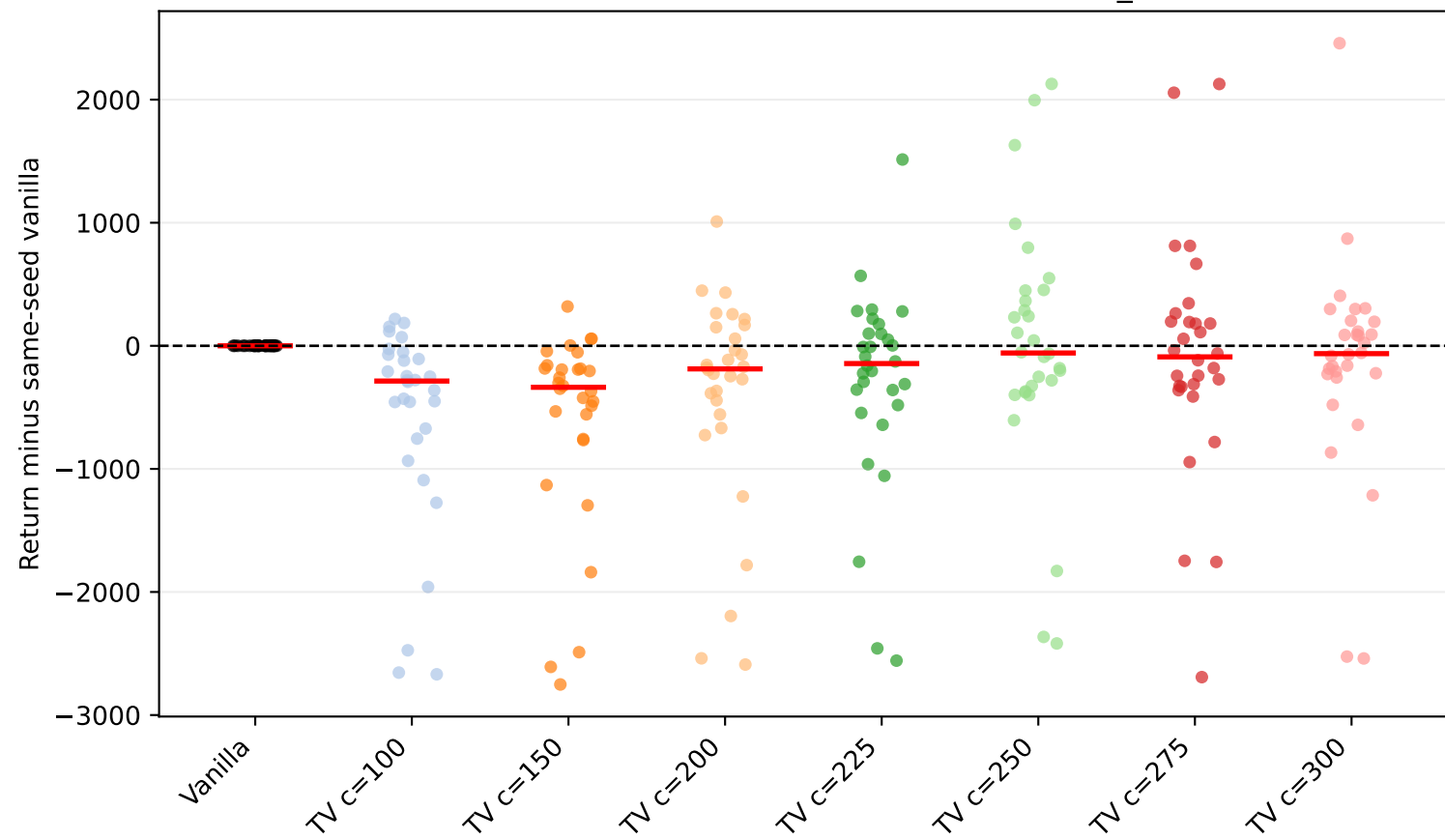
Walker2d-v4 friction factor=0.5: seed scatter (vanilla_subtracted)
