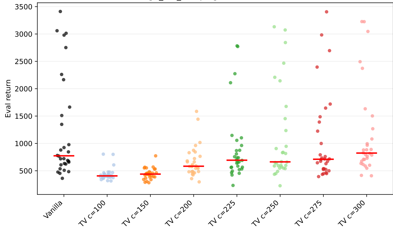
Walker2d-v4 thigh_left_damping factor=0.5: seed scatter (raw)
