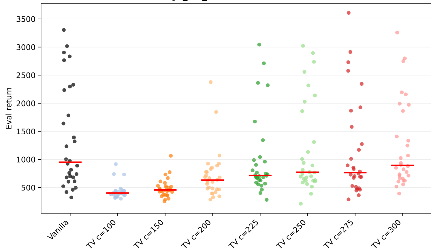
Walker2d-v4 thigh_left_mass factor=0.5: seed scatter (raw)
