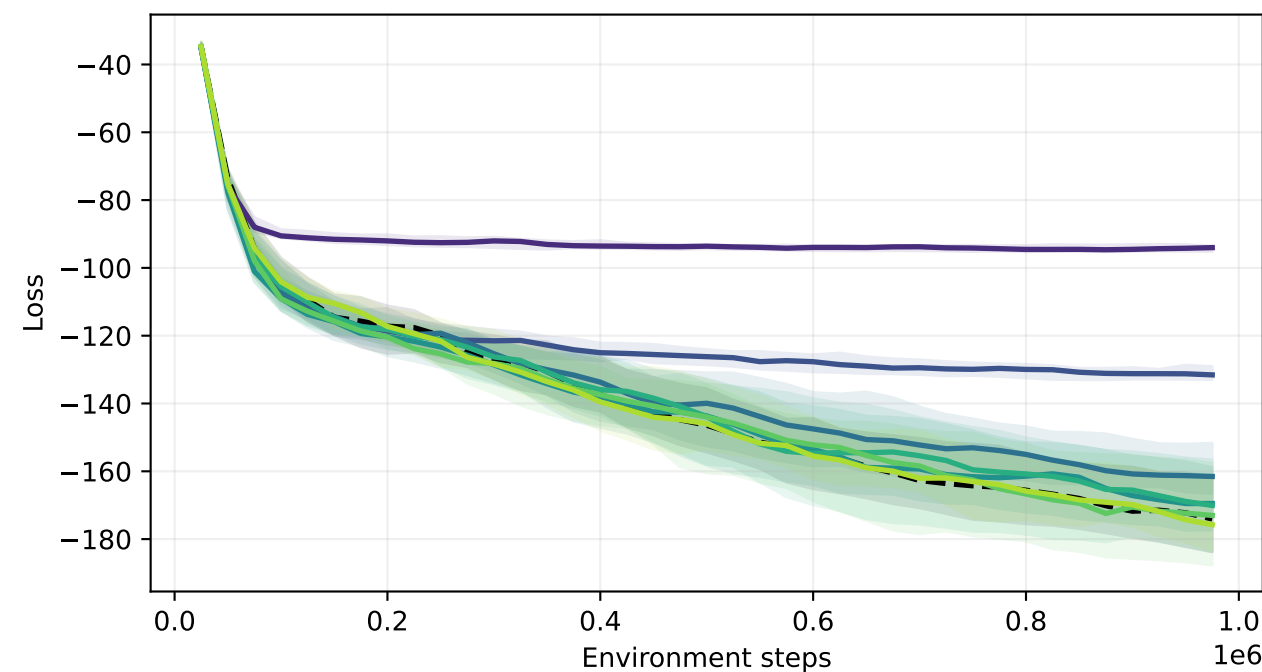
Actor loss
