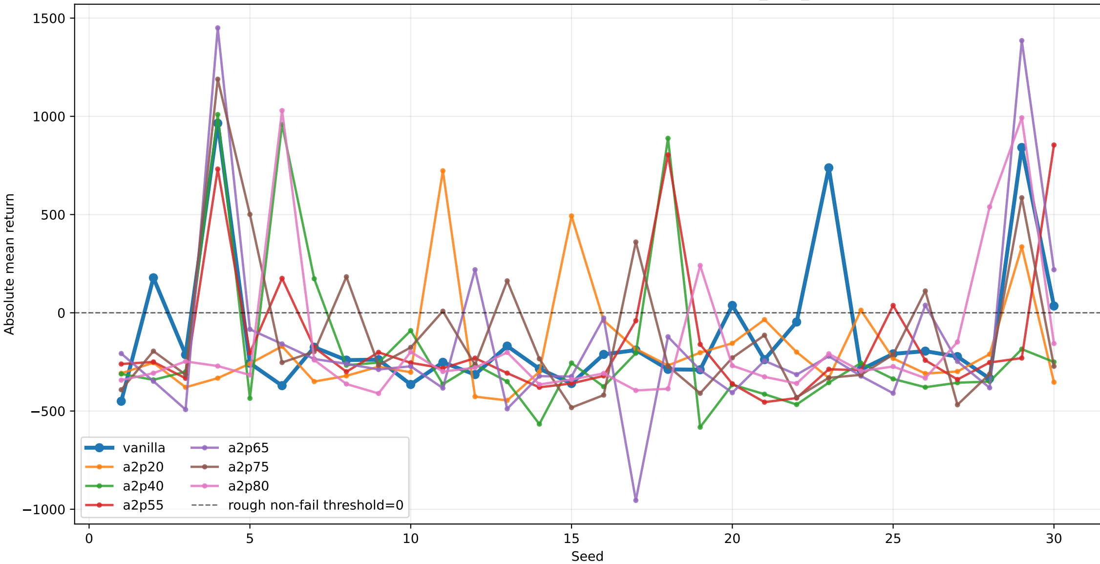
HalfCheetah: absolute returns by seed under actuator_gain_0p5
