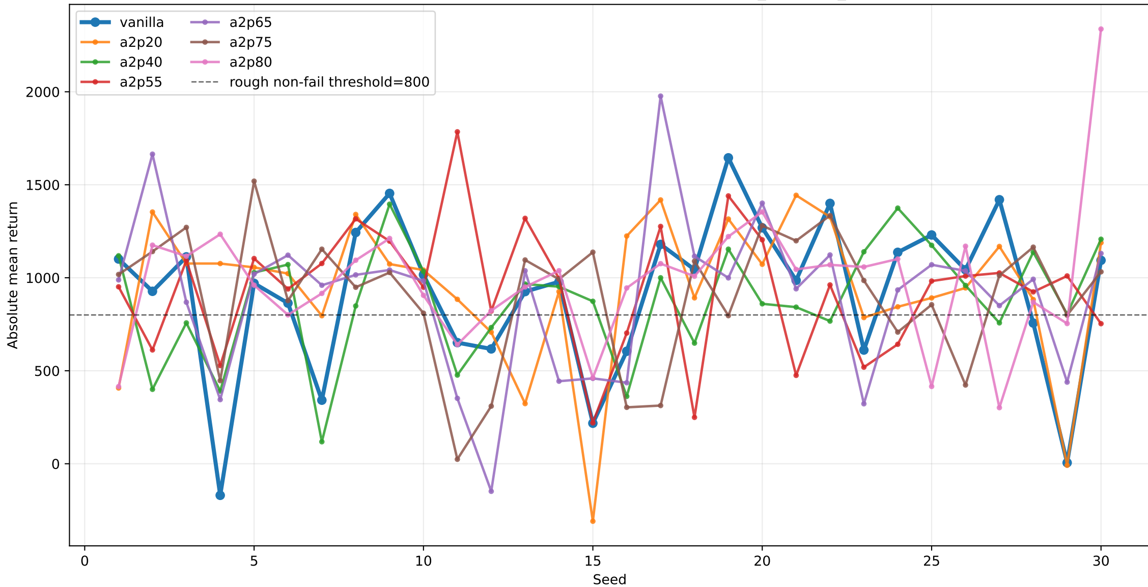
HalfCheetah: absolute returns by seed under mass_damping_0p5
