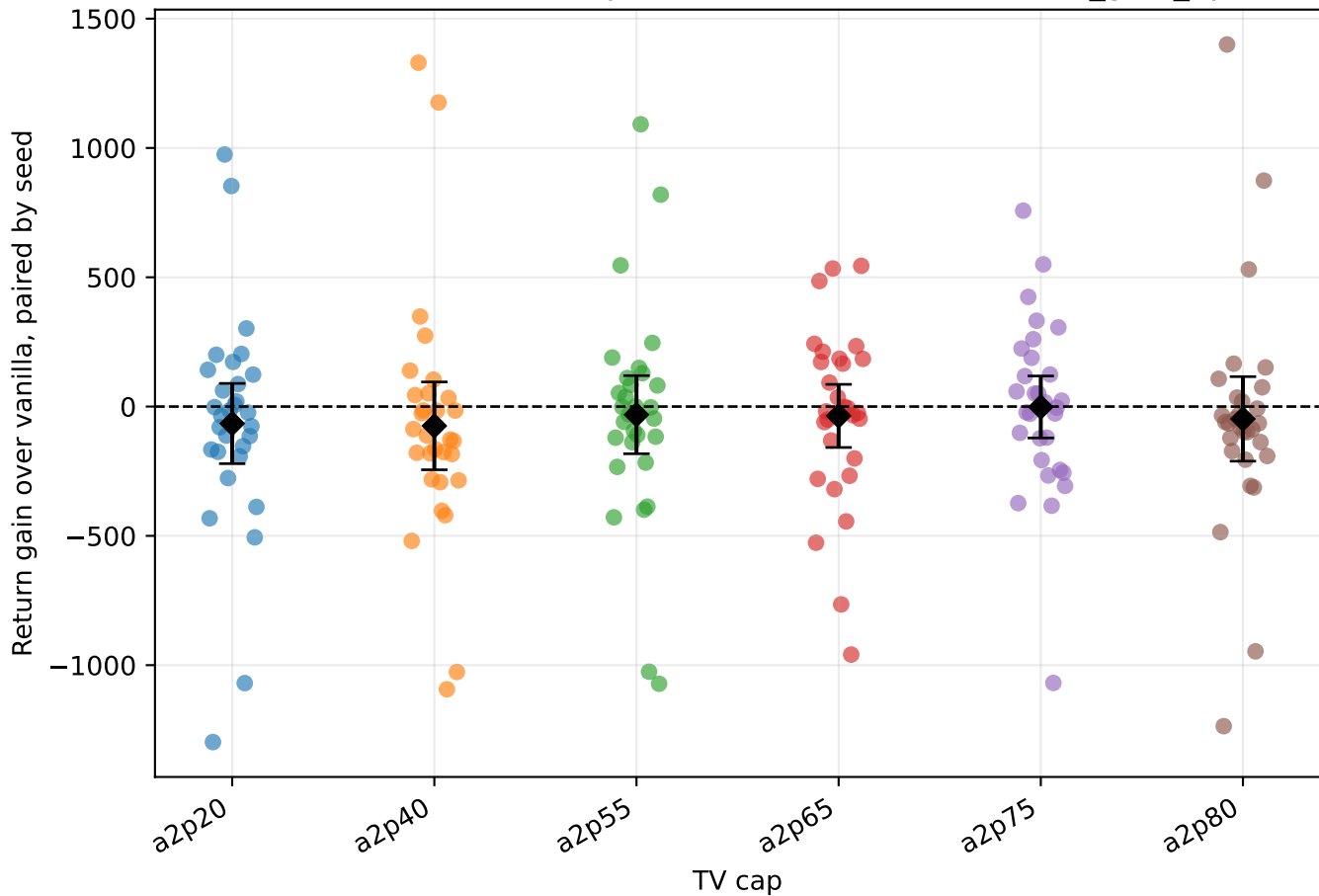
HalfCheetah 30-seed expanded confirmation: actuator_gain_0p5
