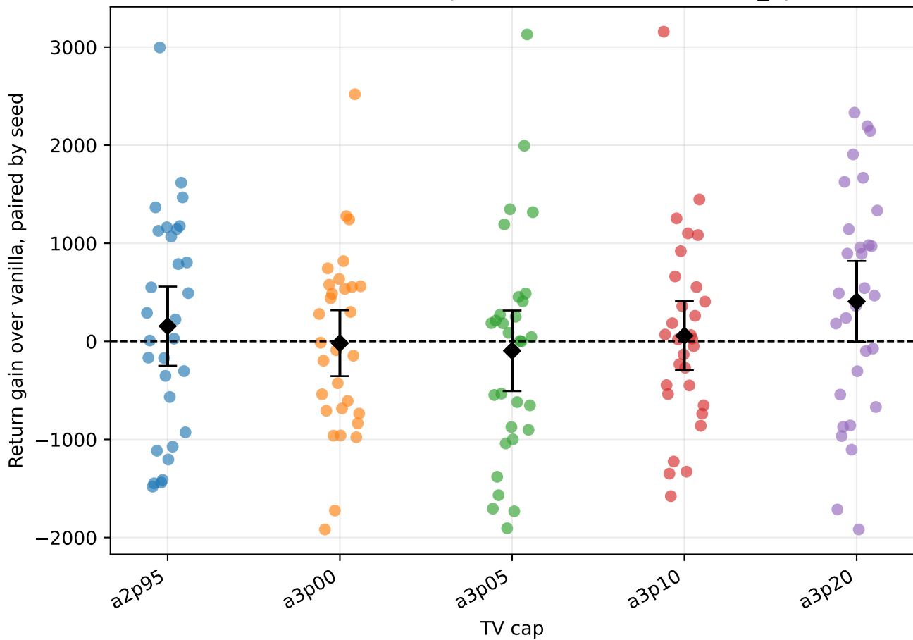
Walker2d 30-seed expanded confirmation: mass_0p5
