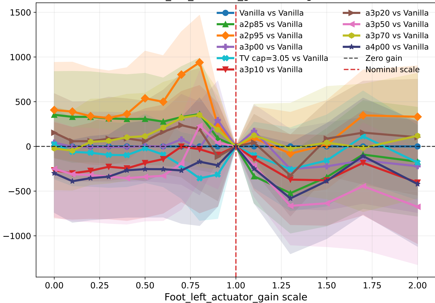
Foot_left_actuator_gain robust gain
