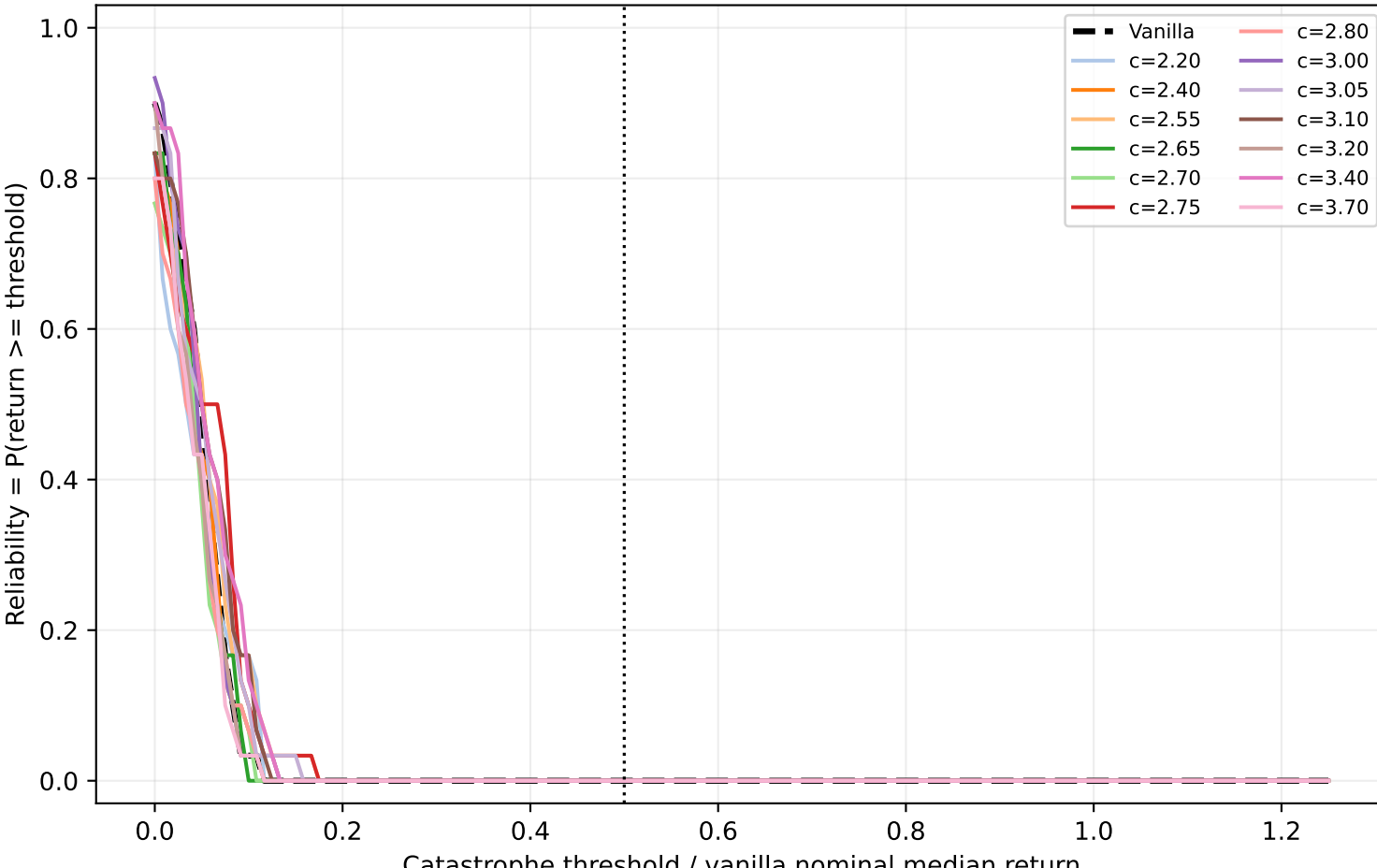
HalfCheetah-v4 action noise bernoulli factor=0.5: robustness reliability curve
