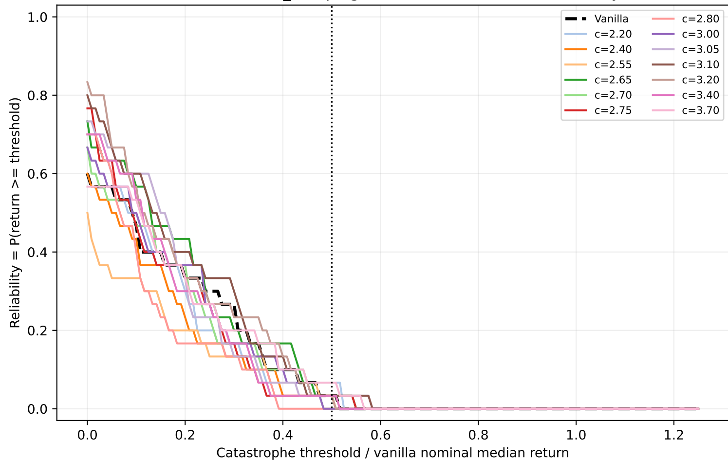
HalfCheetah-v4 mass_damping factor=0.5: robustness reliability curve
