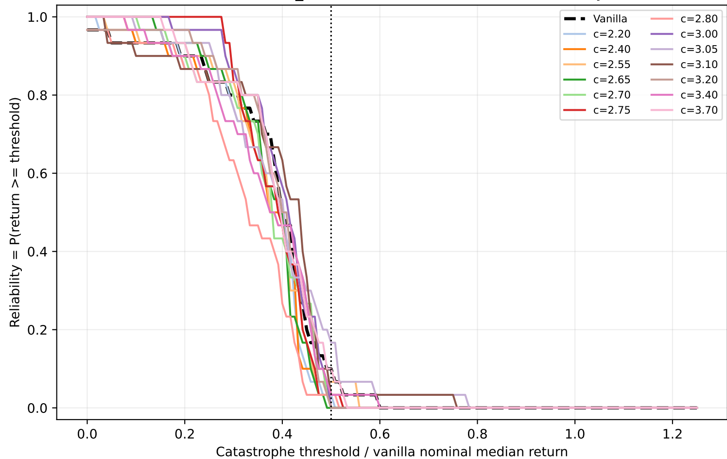
HalfCheetah-v4 state_noise factor=0.5: robustness reliability curve
