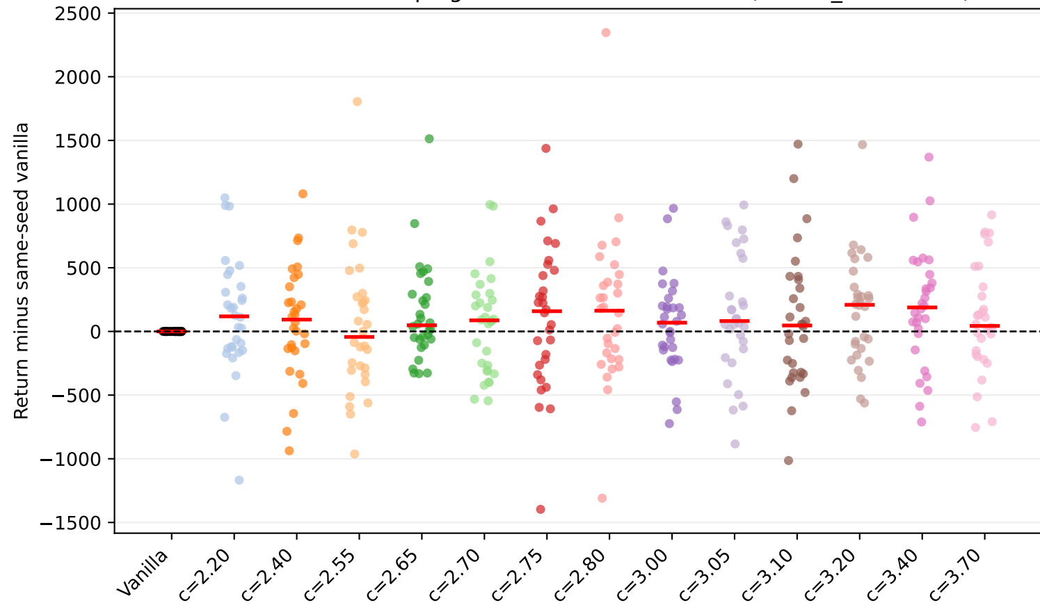
HalfCheetah-v4 damping factor=0.5: seed scatter (vanilla_subtracted)
