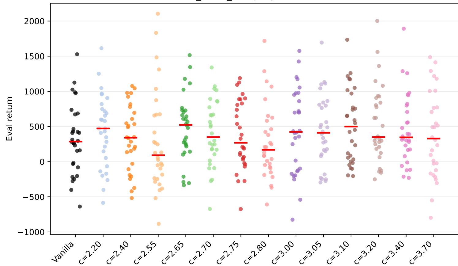
HalfCheetah-v4 friction_mass_damping factor=0.5: seed scatter (raw)
