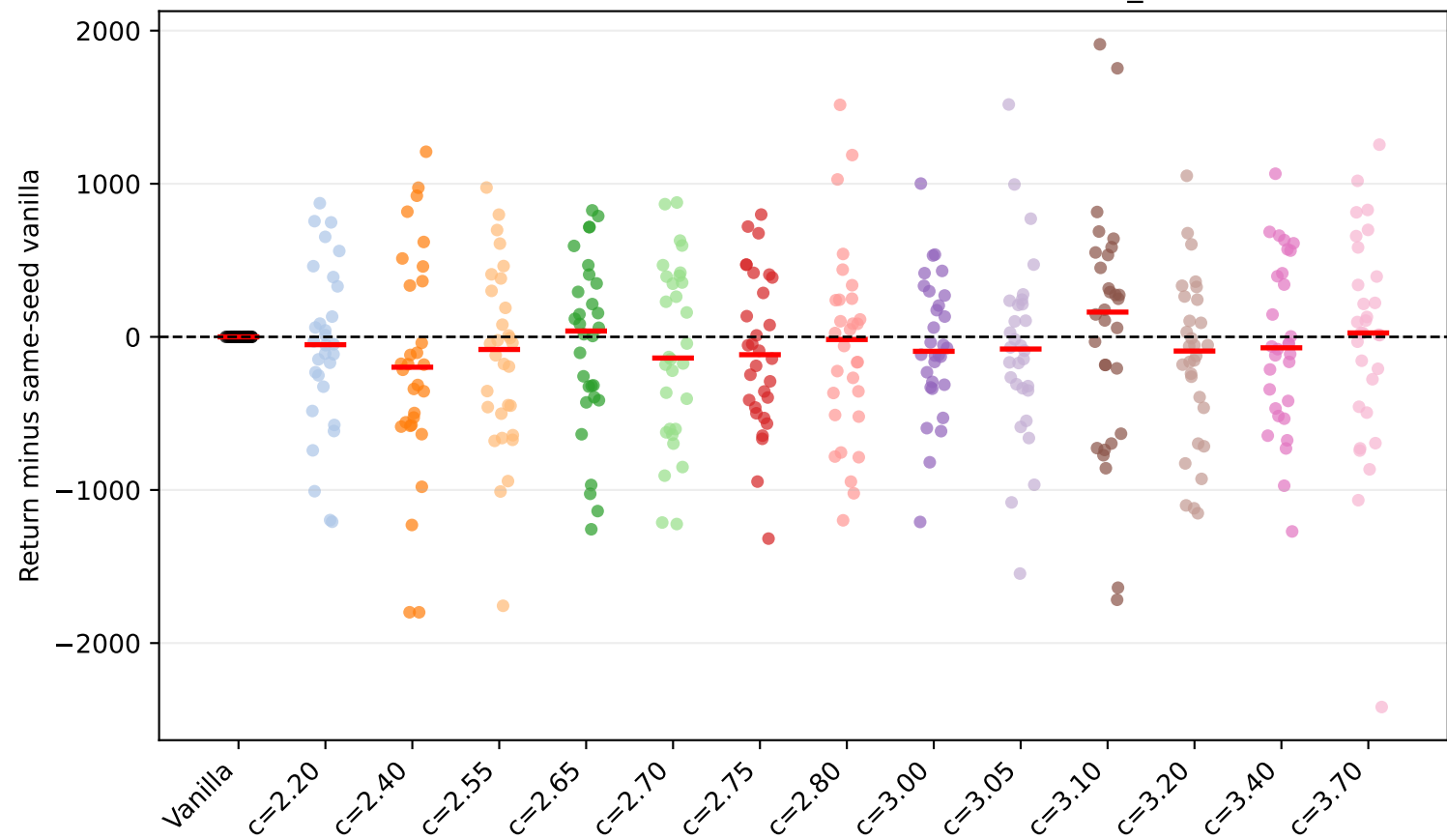
HalfCheetah-v4 mass factor=0.5: seed scatter (vanilla_subtracted)
