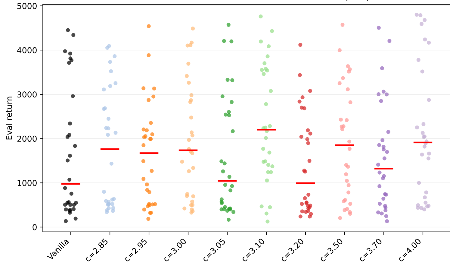
Walker2d-v4 friction factor=0.5: seed scatter (raw)
