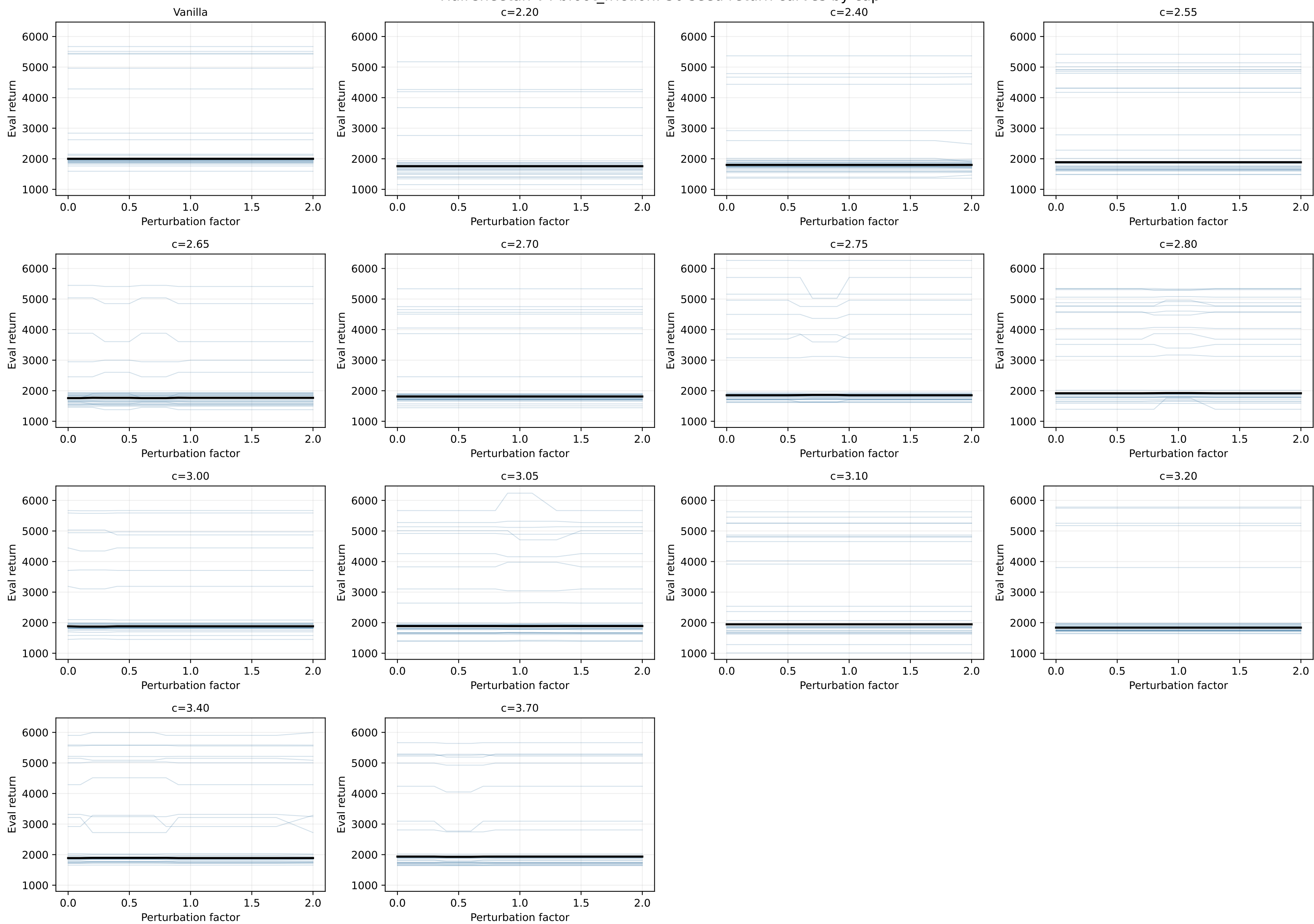
HalfCheetah-v4 bfoot_friction: 30 seed return curves by cap
