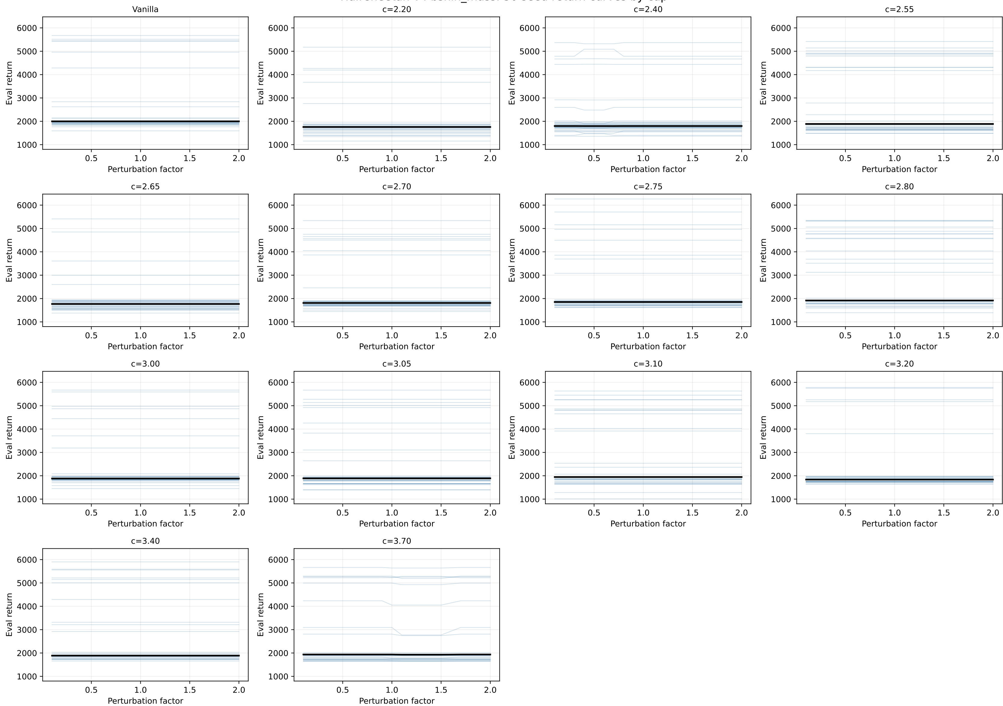
HalfCheetah-v4 bshin_mass: 30 seed return curves by cap
