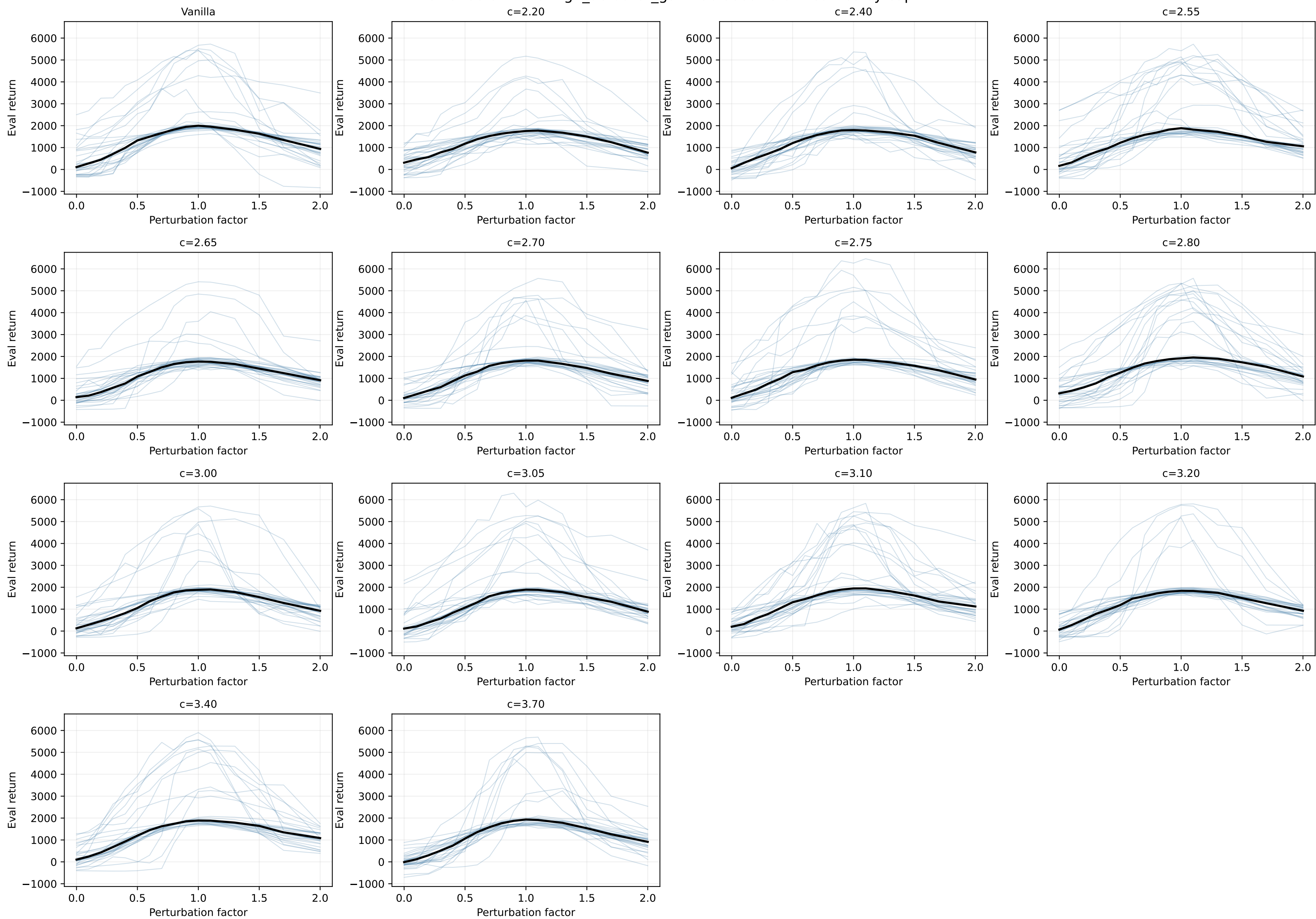
HalfCheetah-v4 bthigh_actuator_gain: 30 seed return curves by cap
