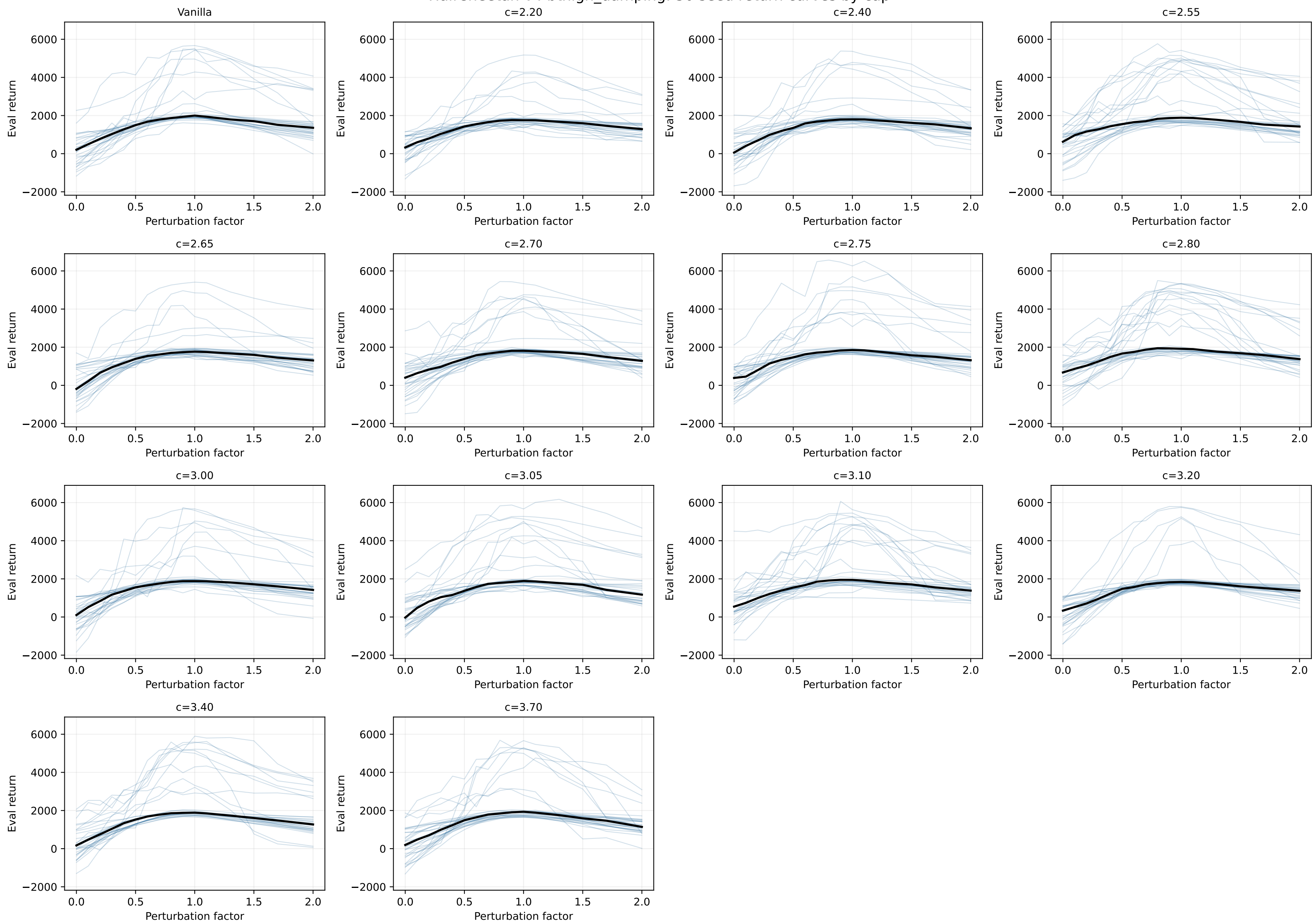
HalfCheetah-v4 bthigh_damping: 30 seed return curves by cap
