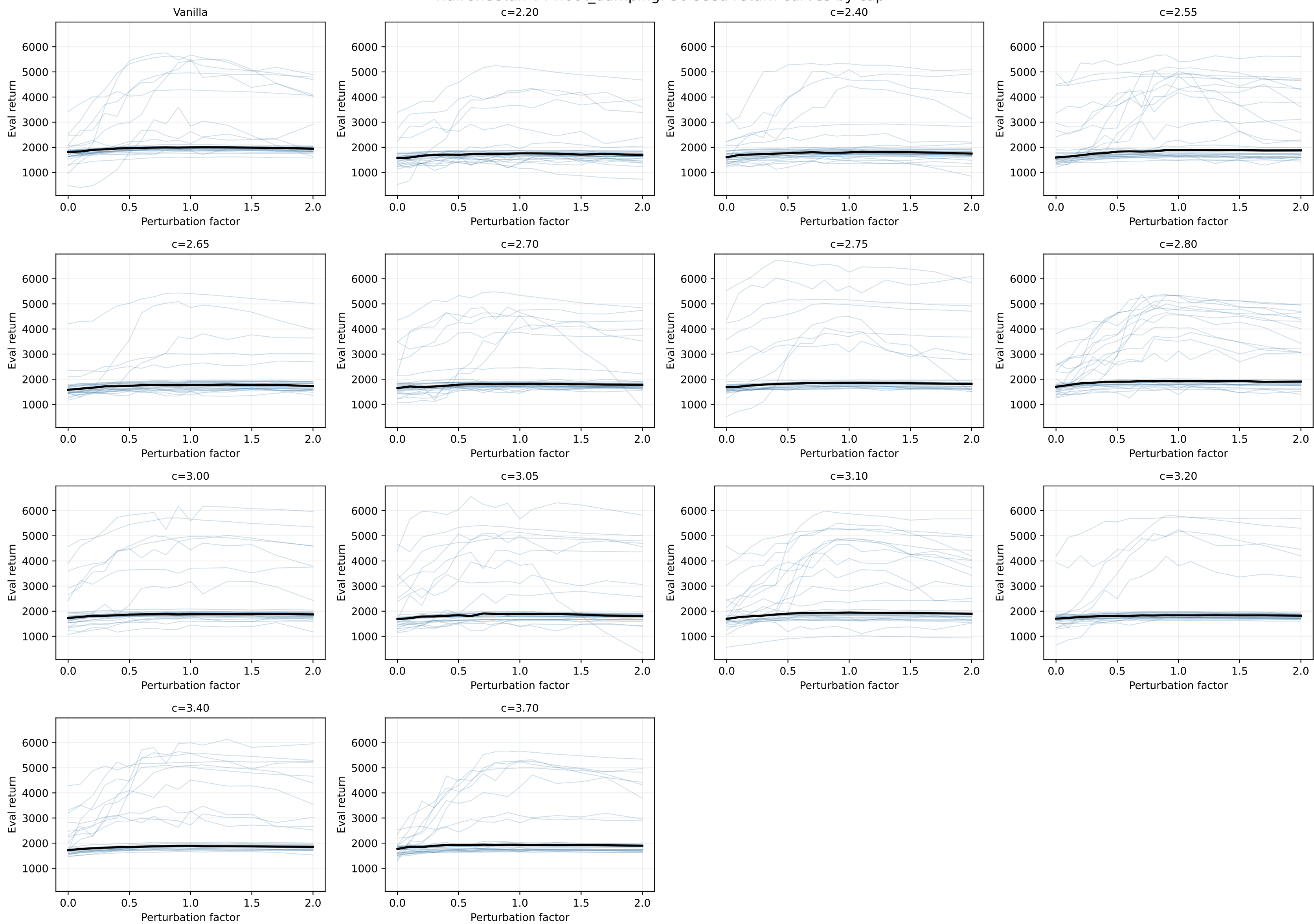
HalfCheetah-v4 ffoot_damping: 30 seed return curves by cap
