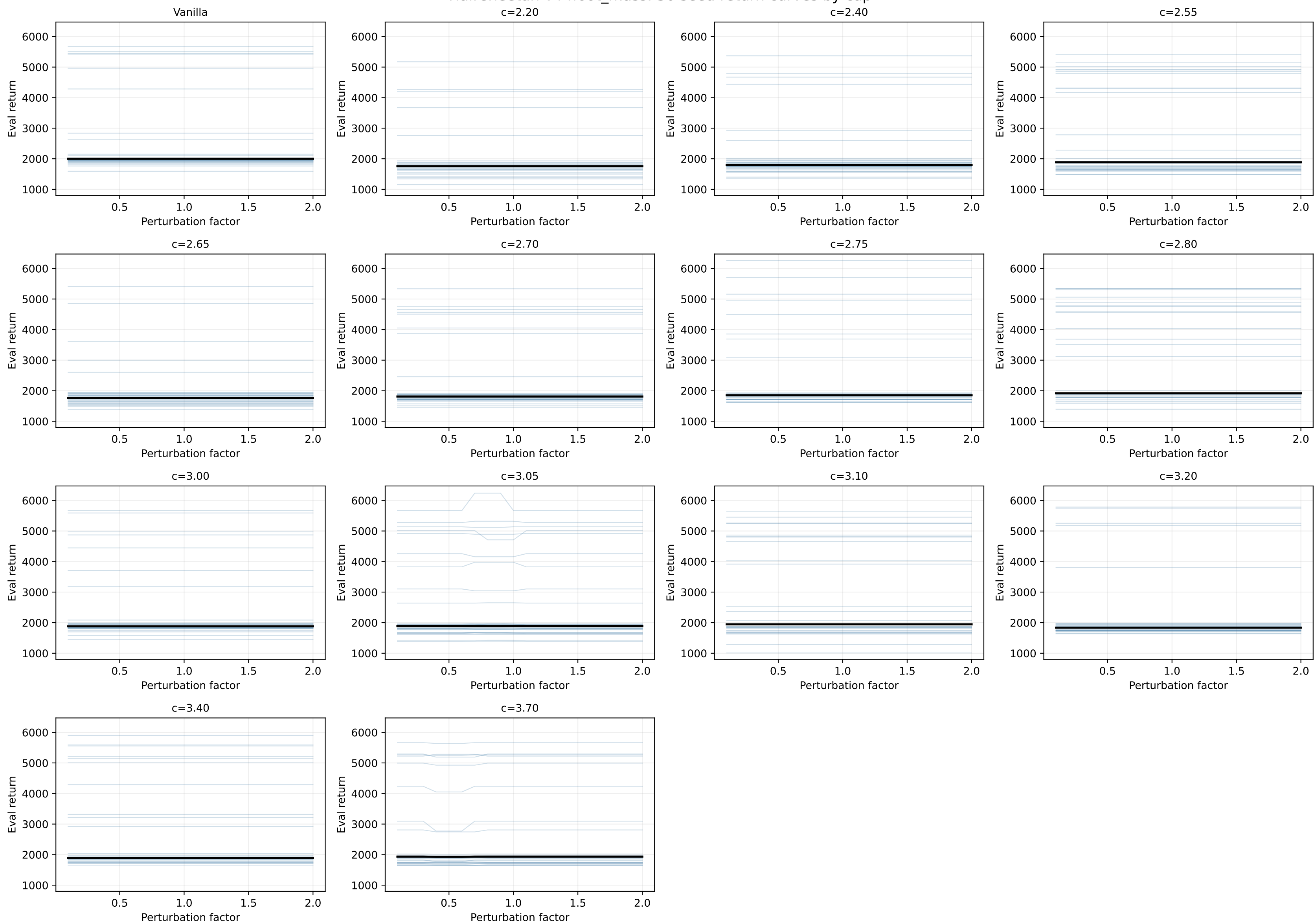
HalfCheetah-v4 ffoot_mass: 30 seed return curves by cap
