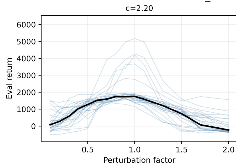
HalfCheetah-v4 friction_mass: 30 seed return curves by cap
