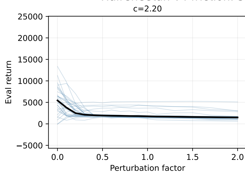
HalfCheetah-v4 friction: 30 seed return curves by cap
