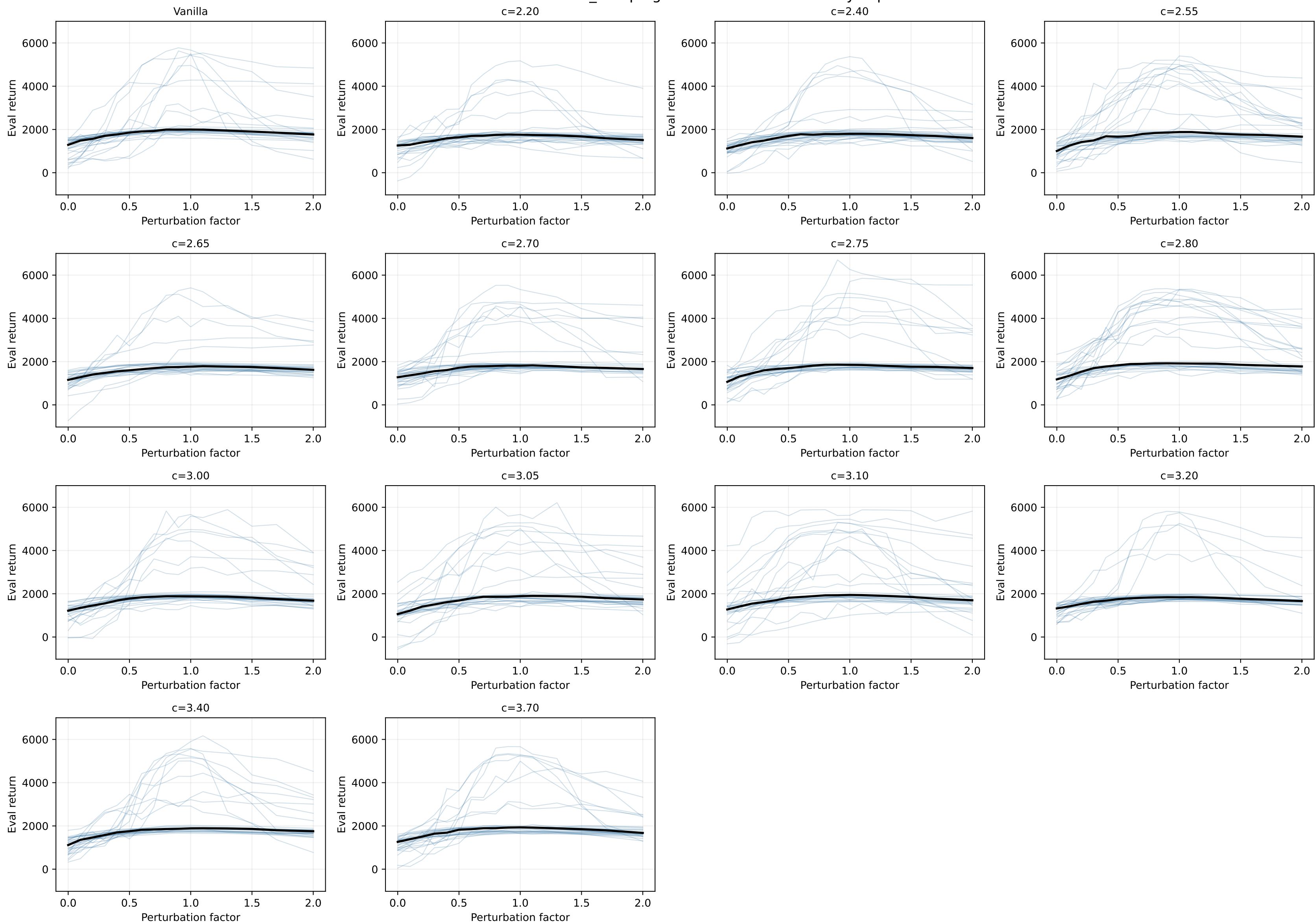
HalfCheetah-v4 fshin_damping: 30 seed return curves by cap
