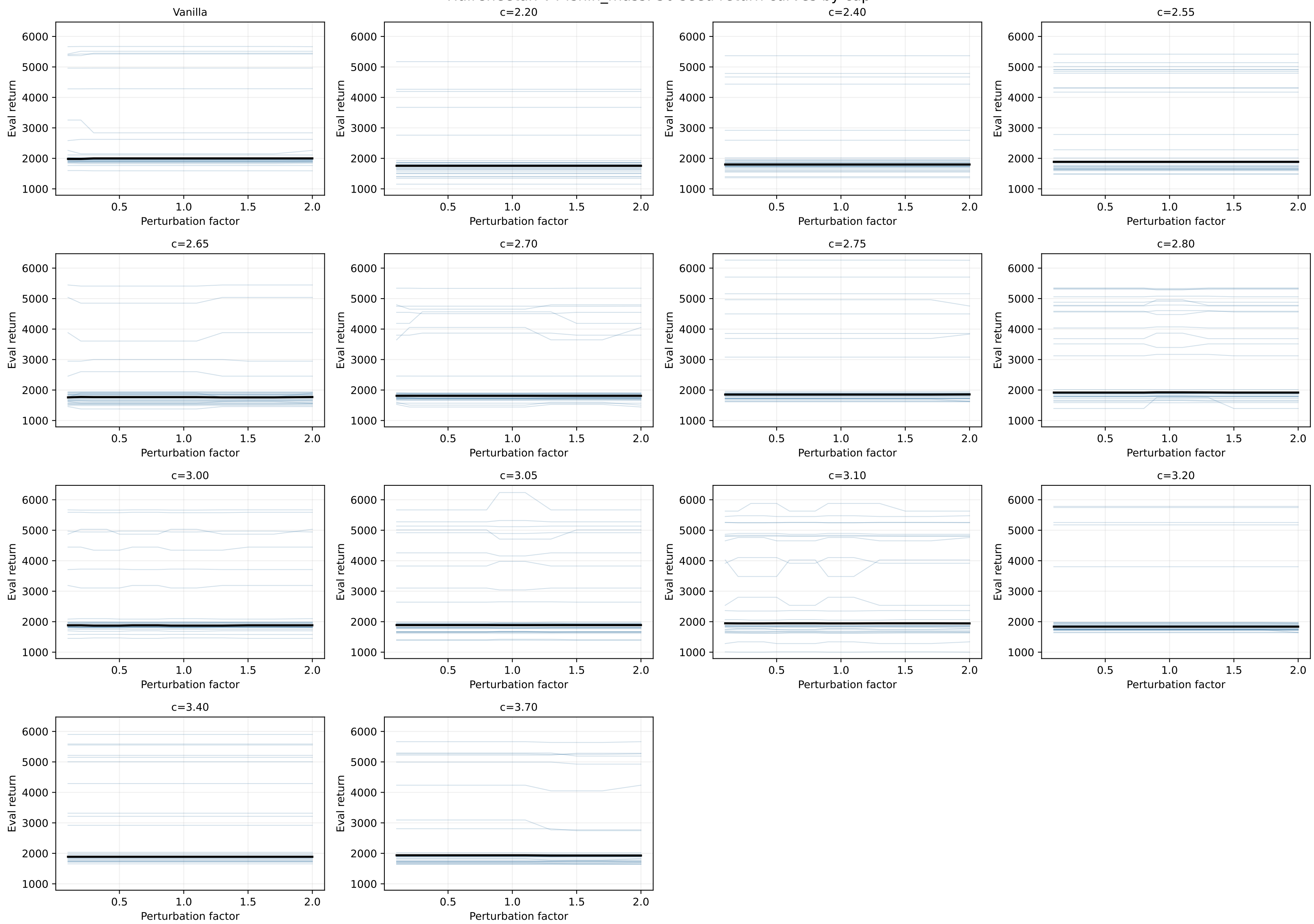
HalfCheetah-v4 fshin_mass: 30 seed return curves by cap
