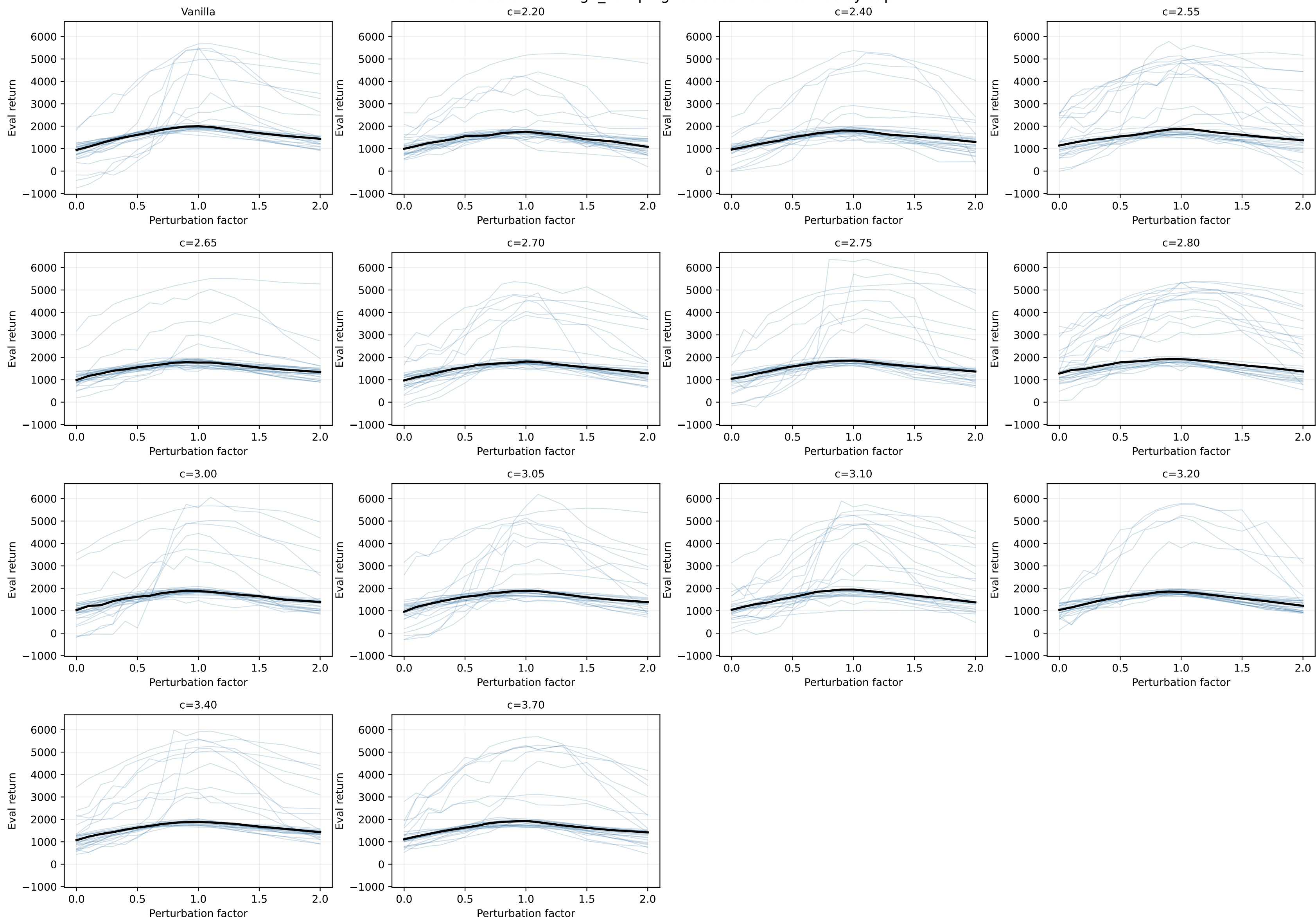
HalfCheetah-v4 fthigh_damping: 30 seed return curves by cap
