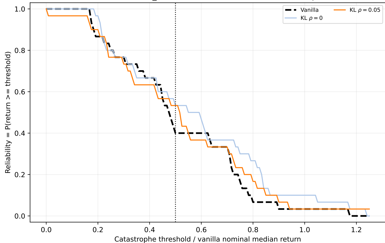
Walker2d-v5 action_noise=0.5: robustness reliability curve
