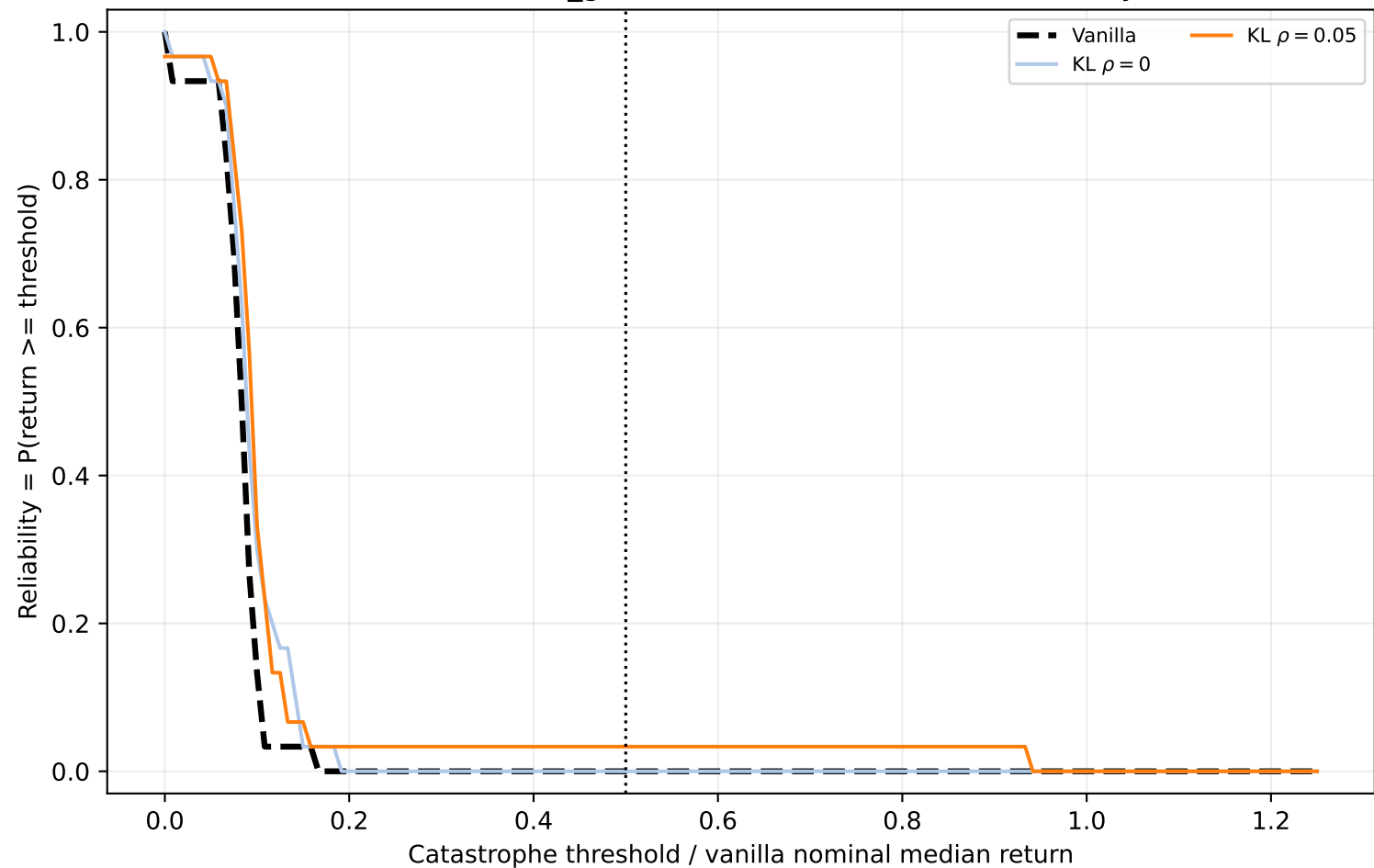
Walker2d-v5 actuator_gain factor=0.5: robustness reliability curve
