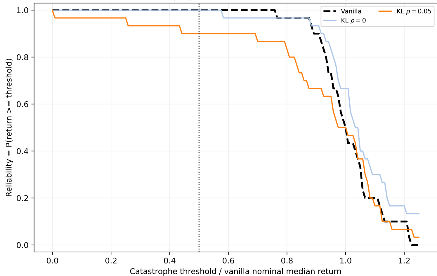
Walker2d-v5 damping factor=0.5: robustness reliability curve
