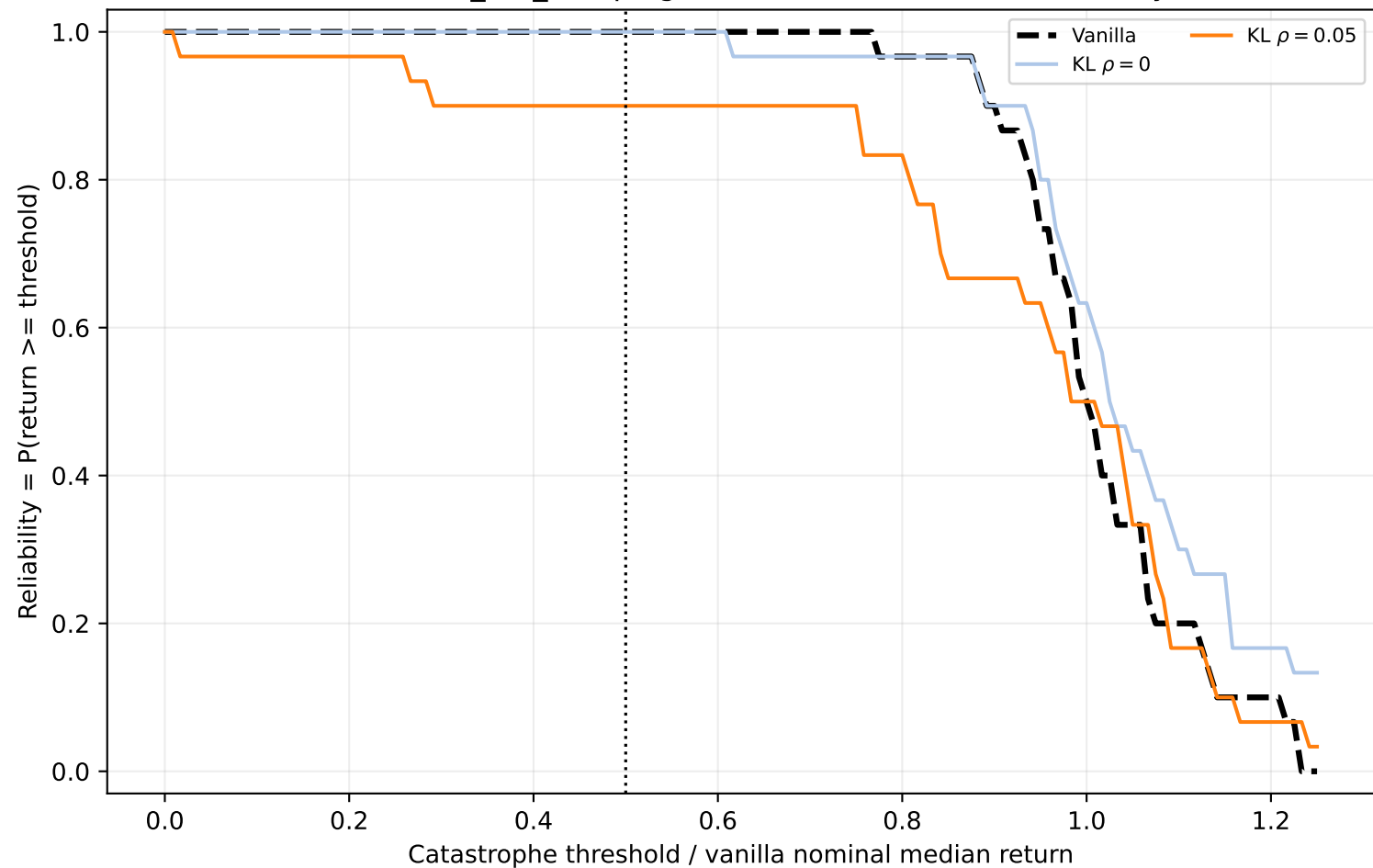
Walker2d-v5 foot_left_damping factor=0.5: robustness reliability curve
