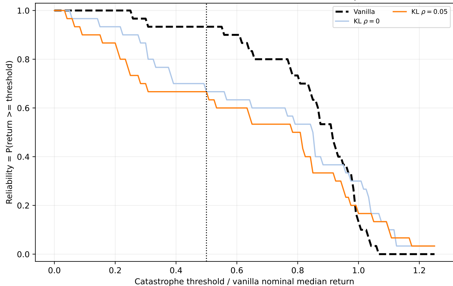
Walker2d-v5 friction factor=0.5: robustness reliability curve
