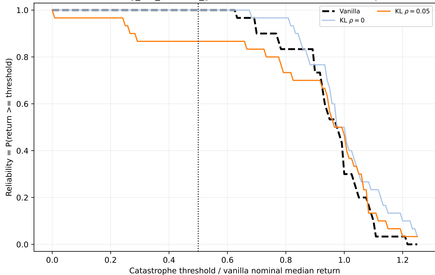
Walker2d-v5 leg_left_actuator_gain factor=0.5: robustness reliability curve
