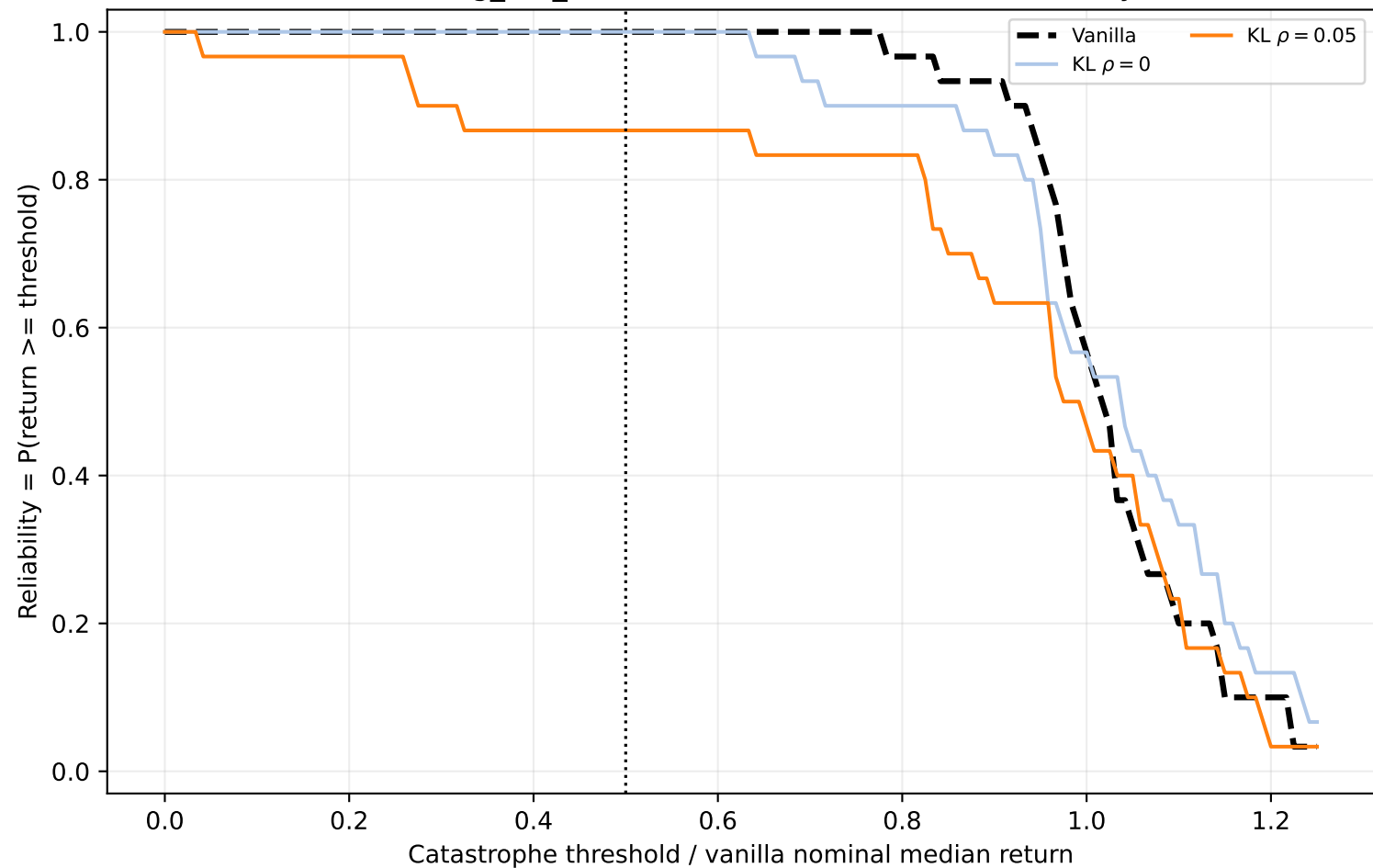
Walker2d-v5 leg_left_mass factor=0.5: robustness reliability curve
