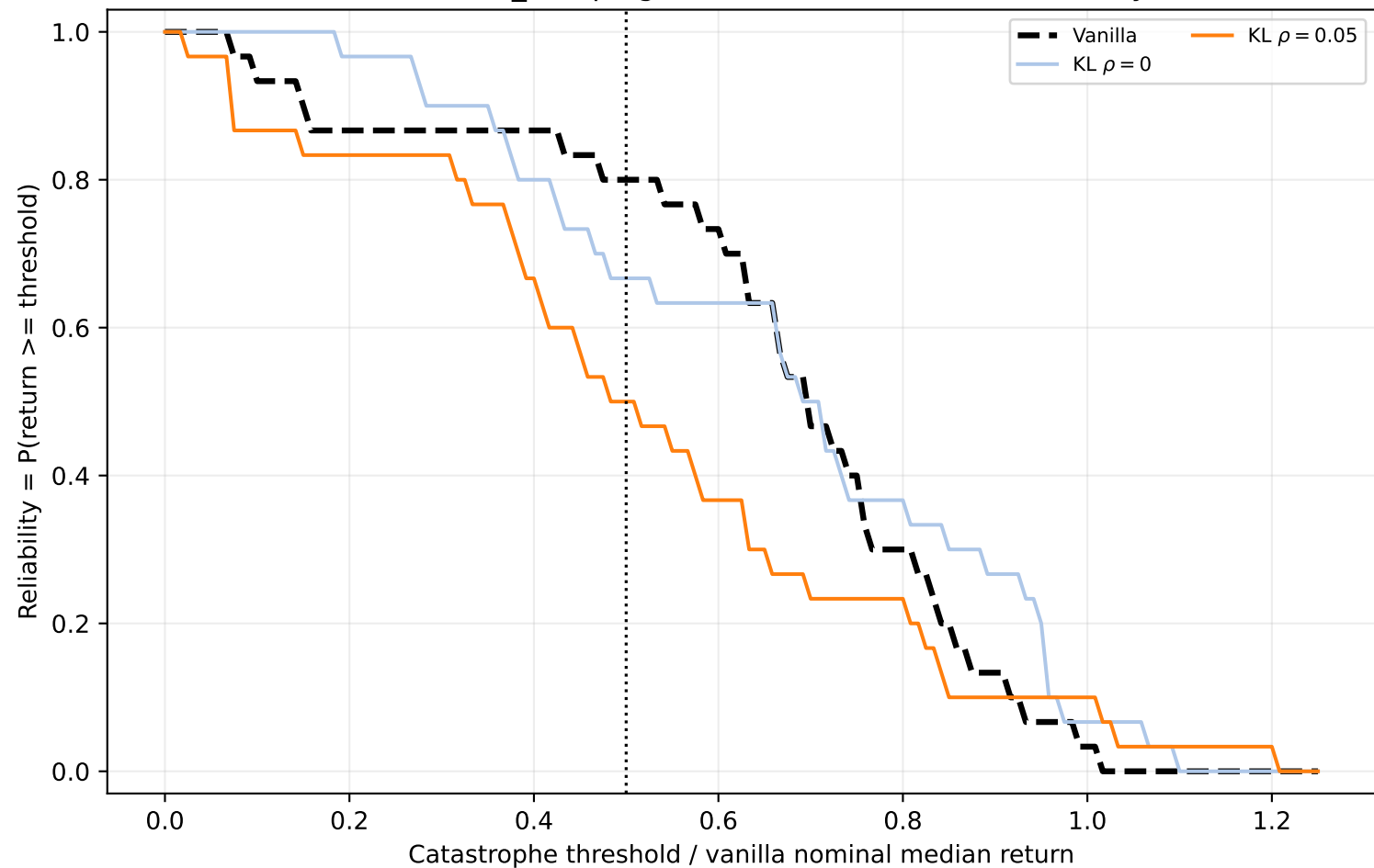
Walker2d-v5 mass_damping factor=0.5: robustness reliability curve
