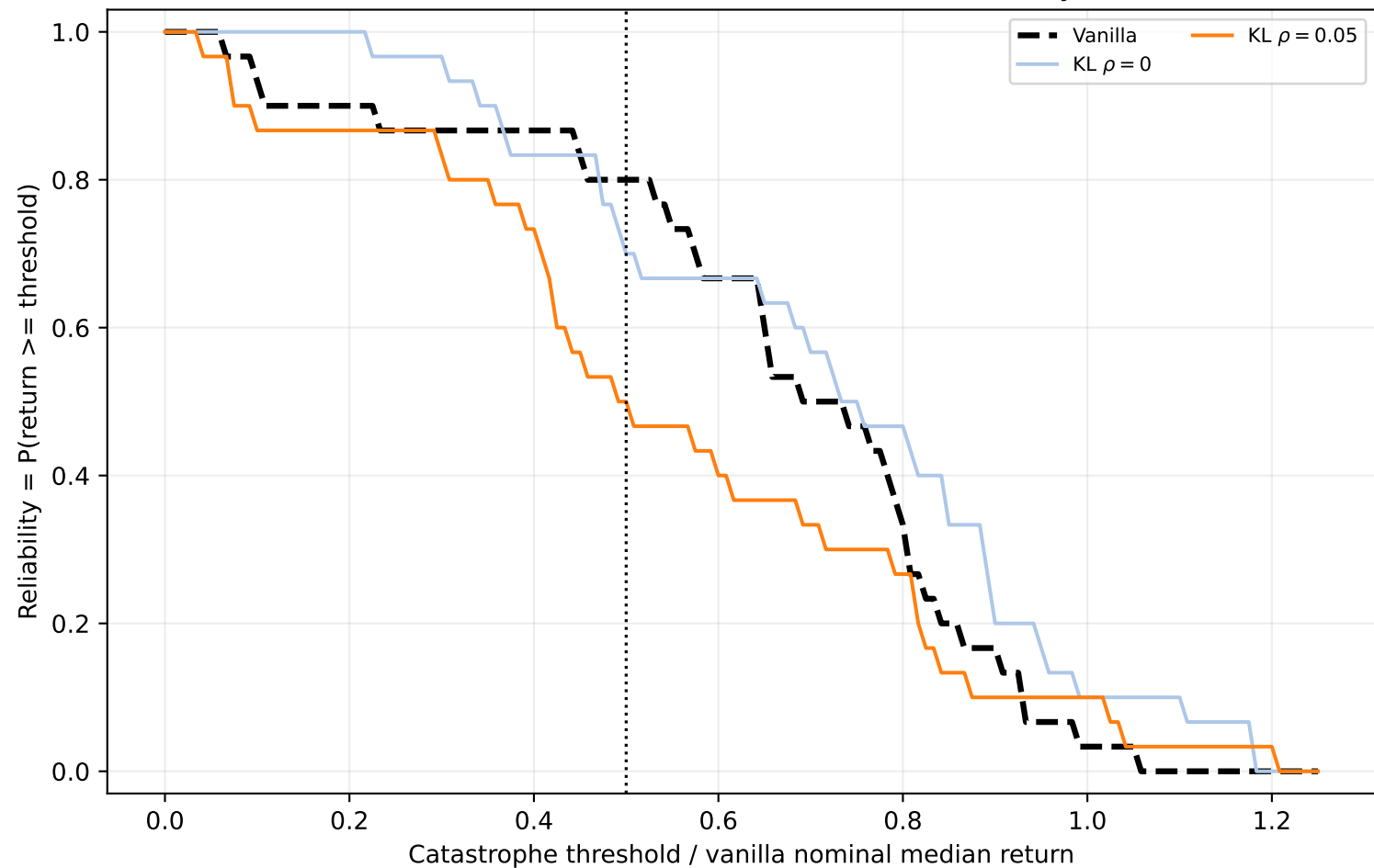
Walker2d-v5 mass factor=0.5: robustness reliability curve
