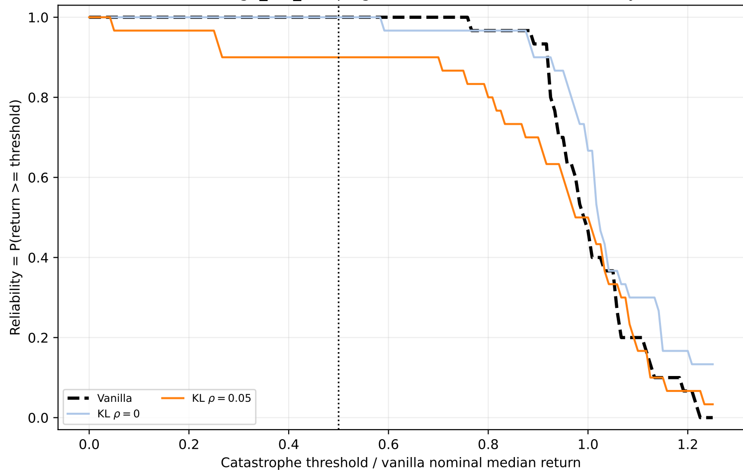
Walker2d-v5 thigh_left_damping factor=0.5: robustness reliability curve
