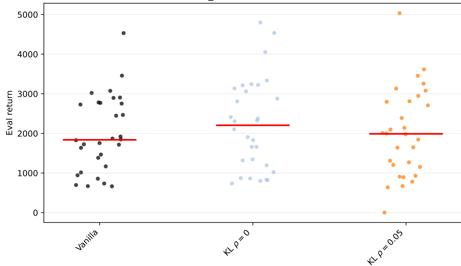
Walker2d-v5 action_noise=0.5: seed scatter (raw)
